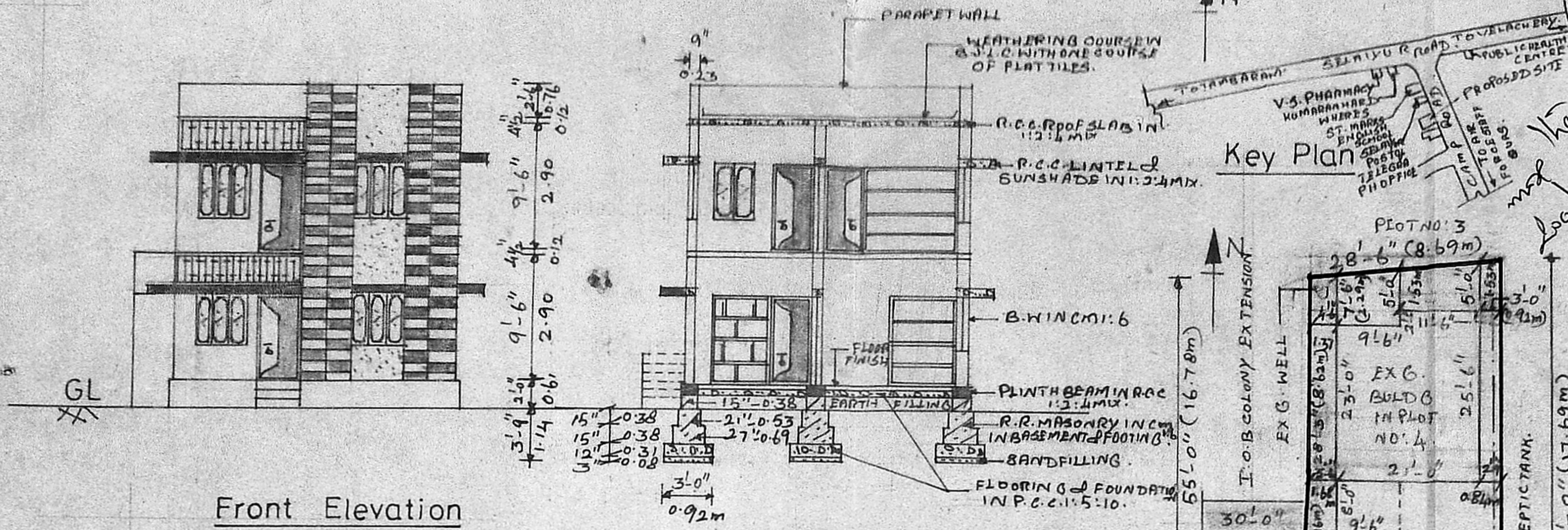
Section On XY
